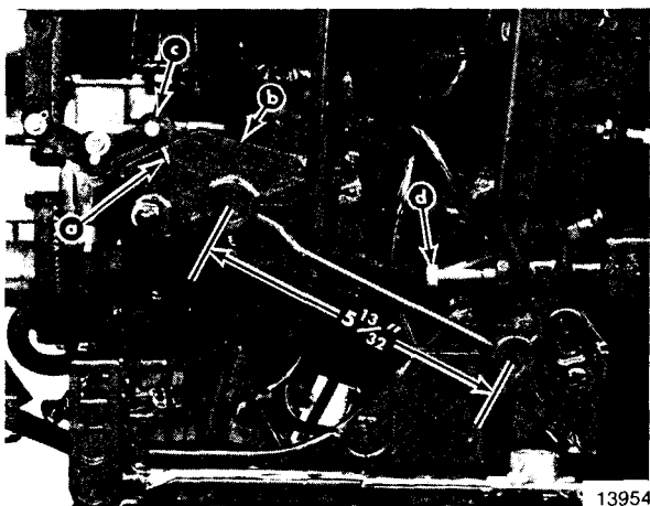
a - Slash Mark b - Throttle Cam c - Roller d - Idle Stop Screw (Adjust so that Slash Mark Is at Point of Contact with Roller)
