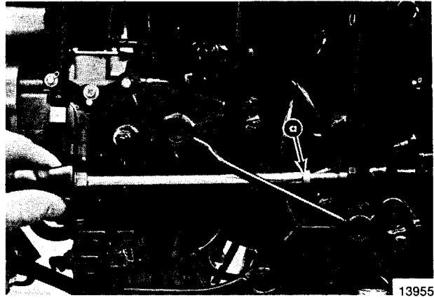
Figure 8. Idle RPM Adjustment
