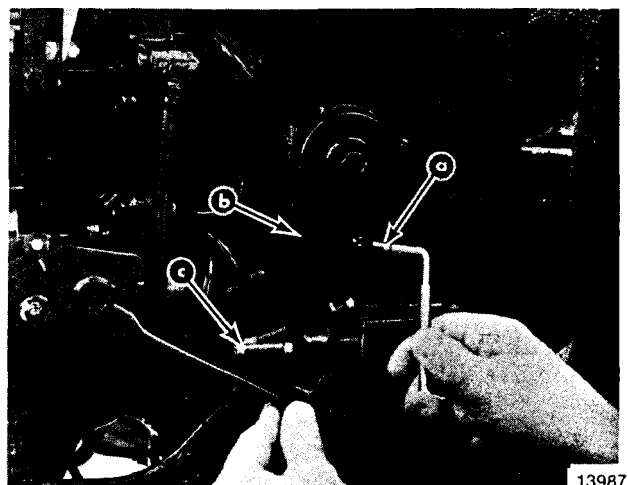
a - Primary Pickup Screw b - Throttle Lever c - Idle Stop Screw (Position against Stop when Adjusting Primary Pickup)
