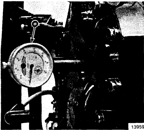
a - Dial Indicator Installed in No. 1 Cylinder
