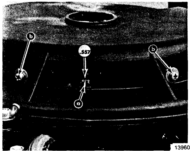
a - Timing Pointer; Align with .557" Mark b - Timing Pointer Attaching Screws
